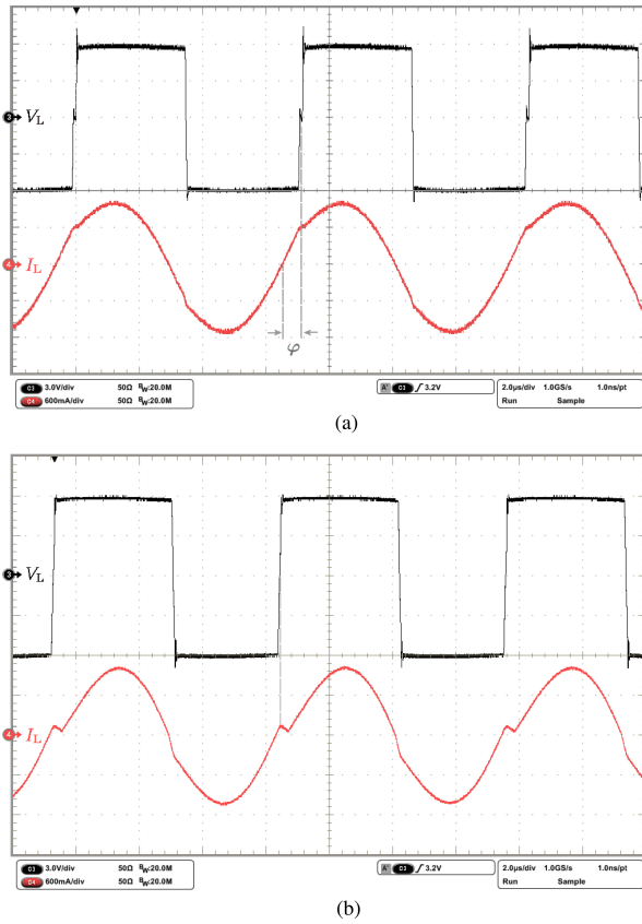
Fig. 9. Measurement of the key system waveforms for the proposed concept and a synchronous rectification approach at k = 0.6 . (a) Waveforms of the rectifier input voltage V_L (3V/div) and input current I_L (600 mA/div) for the proposed concept with a phase-shift of \varphi = 20^\circ and a duty cycle D = 68\% . (b) Waveforms of V_L (3V/div) and I_L (600 mA/div) for synchronous rectification with a duty cycle D = 66\% .
